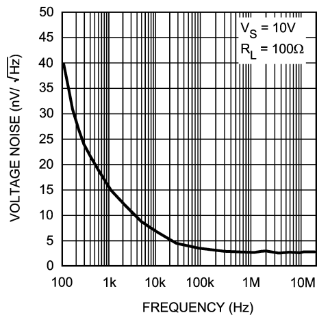
Voltage Noise
