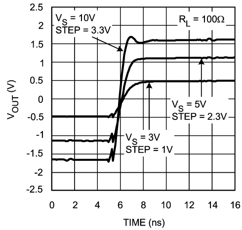
Transient Response Positive for Various V_{SUPPLY}
