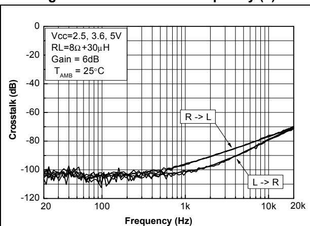
Figure 39. Crosstalk vs. frequency (ii)
