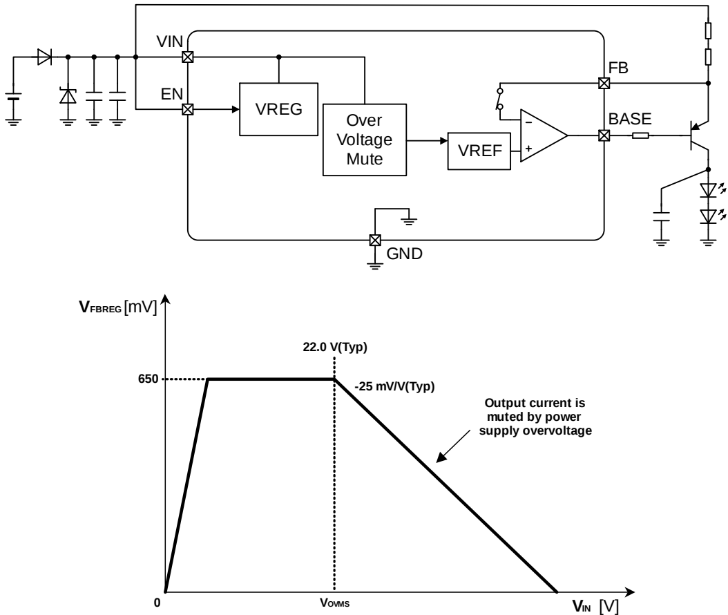
Figure 29. Over Voltage Mute Function (OVM)
