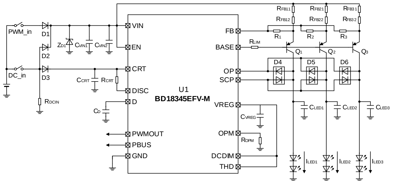
Figure 33. Application Example 3
