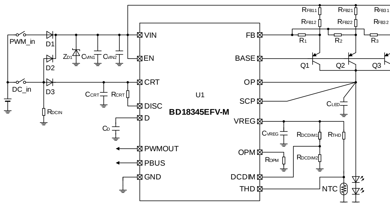
Figure 32. Application Example 2
