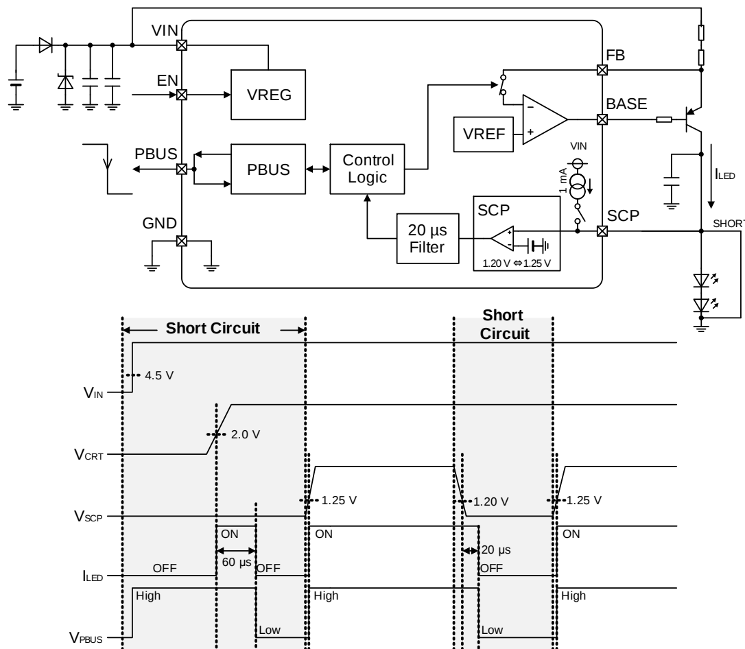
Figure 22. Short Circuit Protection (SCP)
