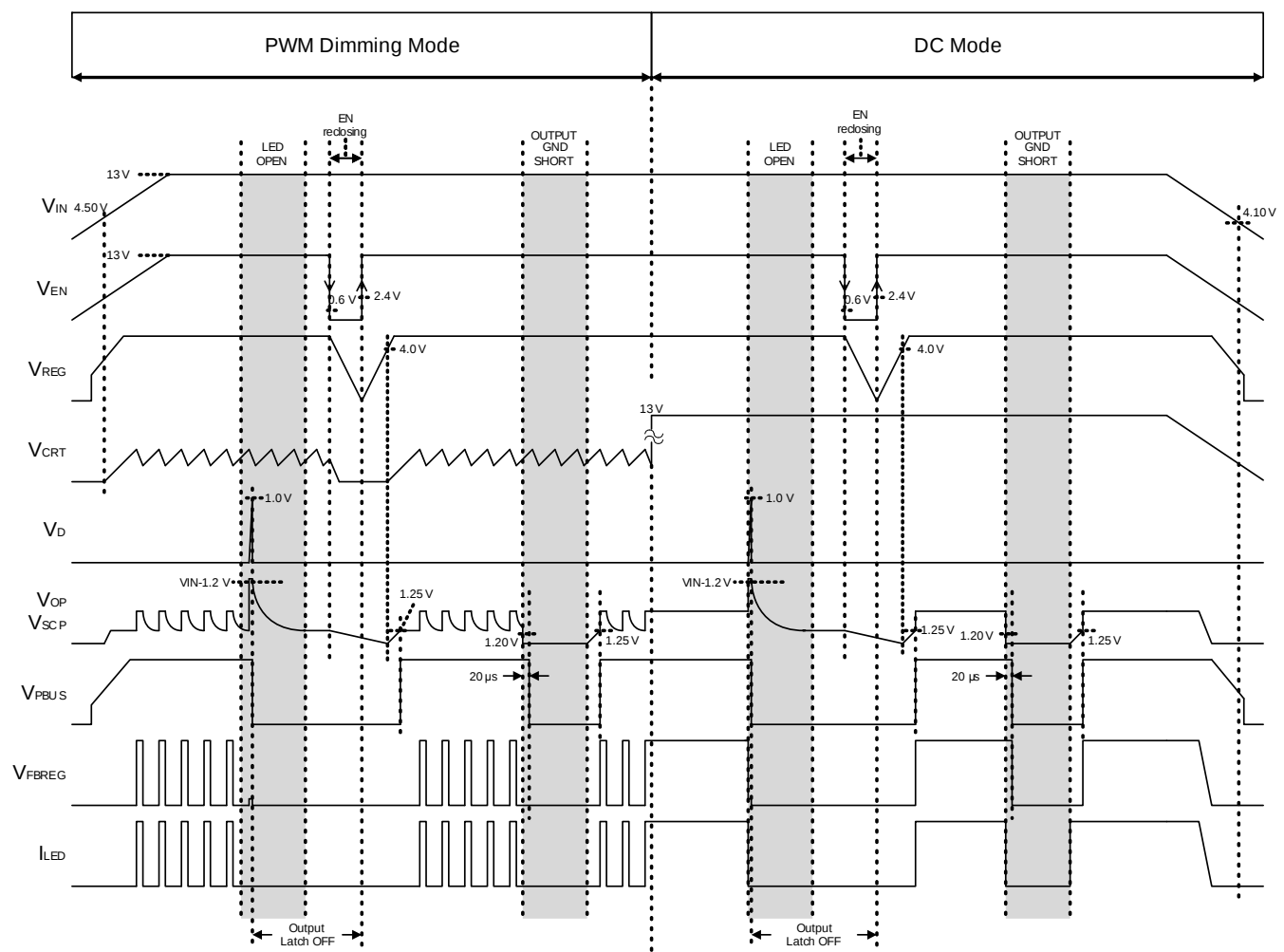
Figure 30. Timing Chart
