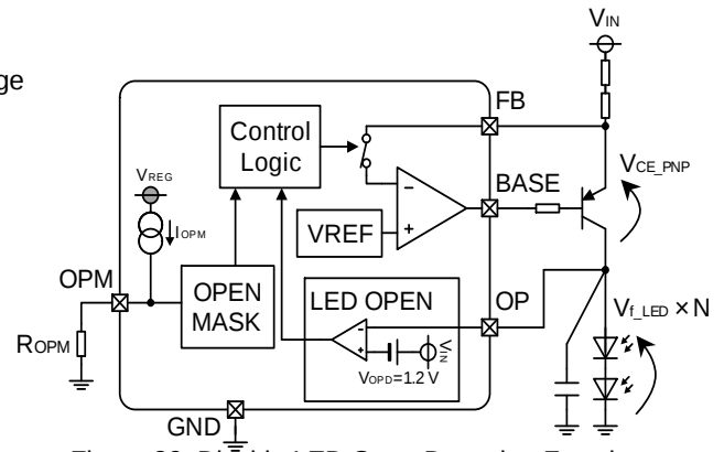
Figure 20. Disable LED Open Detection Function at Reduced-Voltage
