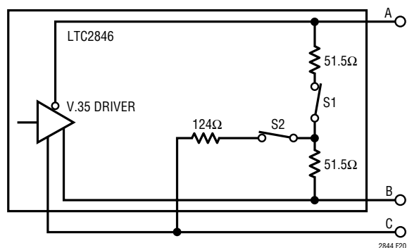
Figure 20. V.35 Driver
