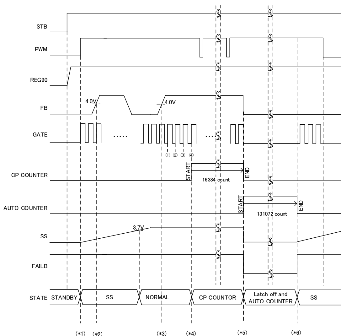
Figure 35. FBMAX Detection
