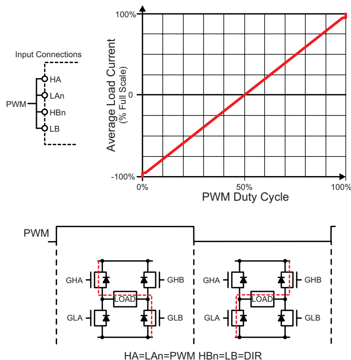
Figure 9: Single PWM Input, Fast Decay, SR
