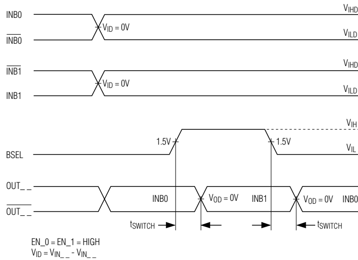
Figure 3. Input to Rising/Falling Edge Select and Mux Switch Timing Diagram
