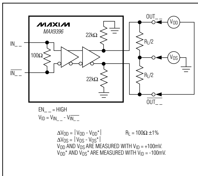
Figure 2. Test Circuit for V_{OD} and V_{OS}
