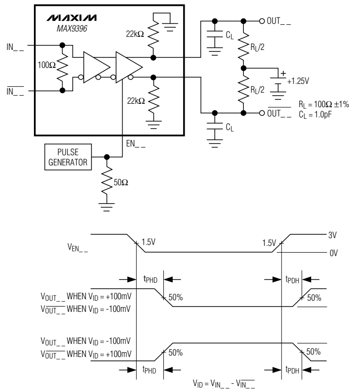
Figure 4. Output Active-to-Disable and Disable-to-Active Test Circuit and Timing Diagram
