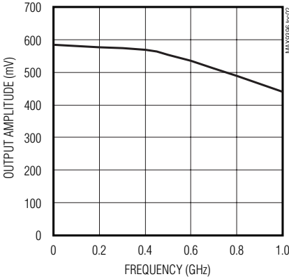
OUTPUT AMPLITUDE vs. FREQUENCY
