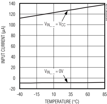
SINGLE-ENDED INPUT CURRENT vs. TEMPERATURE
