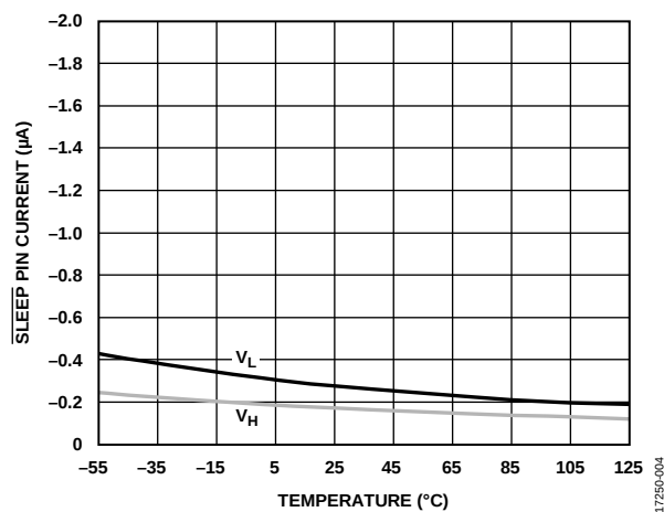
Figure 4. SLEEP Pin Current vs. Temperature
