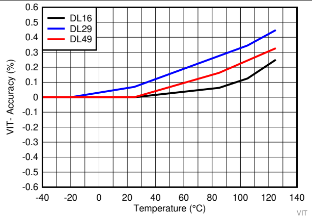
Figure 10. Negative-going Input Threshold Accuracy over Temperature for TPS3840DL-Q1
