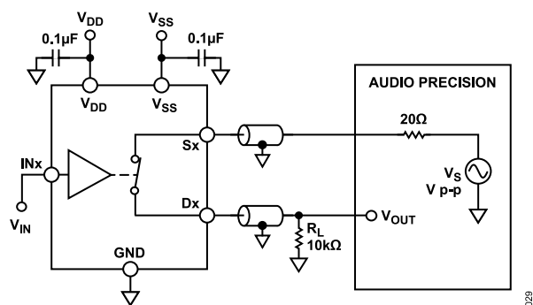
Figure 32. THD + Noise
