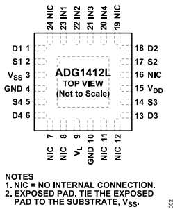
Figure 2. Pin Configuration
