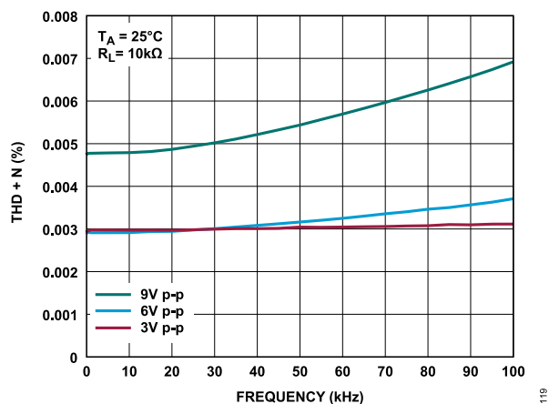
Figure 22. THD + N vs. Frequency, +12 V Single Supply
