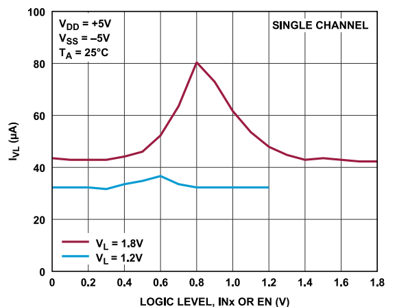
Figure 13. I_{VL} vs. Logic Level
