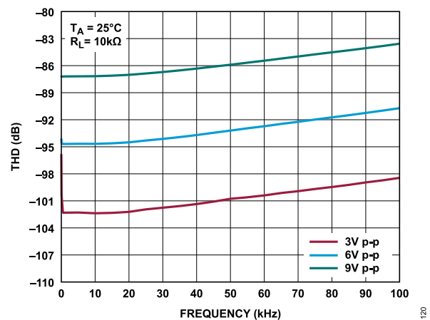
Figure 23. THD vs. Frequency, +12 V Single Supply
