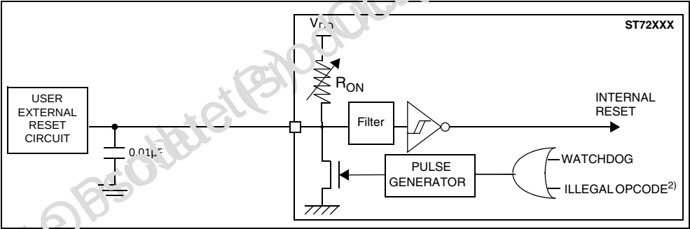
Figure 64. RESET Pin Protection 1)
