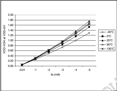
Figure 60. Typical V_{DD}-V_{OH} at V_{DD} = 5V
