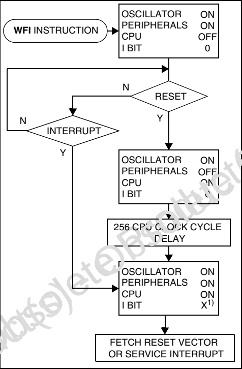
Figure 18. WAIT Mode Flowchart
