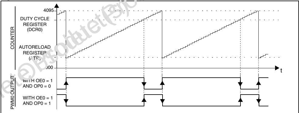
Figure 29. PWM Function
