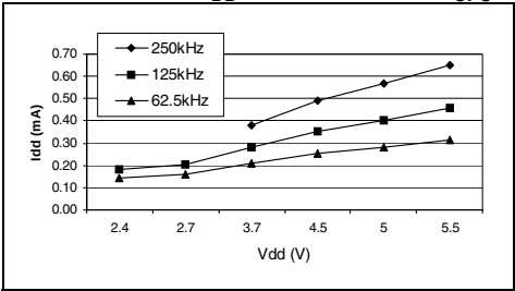
Figure 50. Typical I DD in SLOW WAIT vs f CPU
