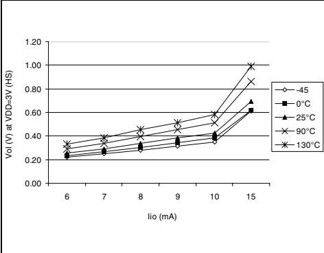
Figure 57. Typical V_{OL} at V_{DD} = 3V (high-sink)
