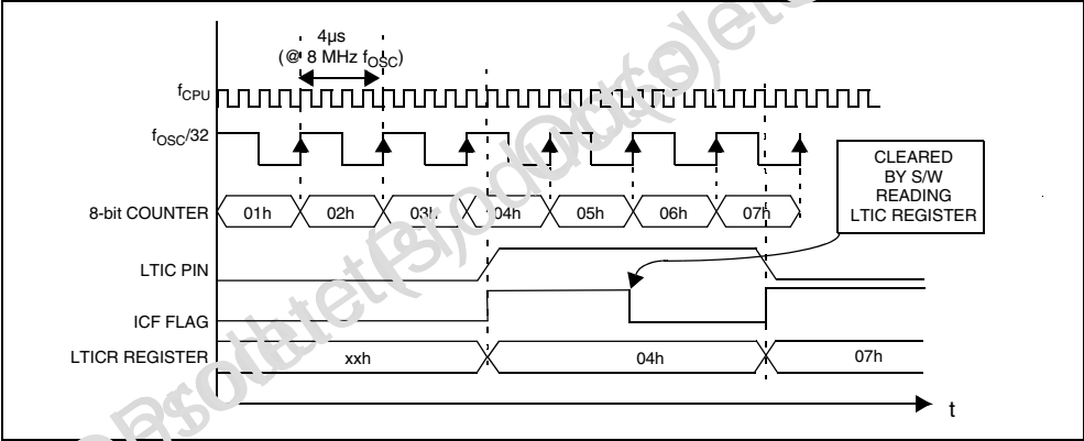
Figure 27. Input Capture Timing Diagram
