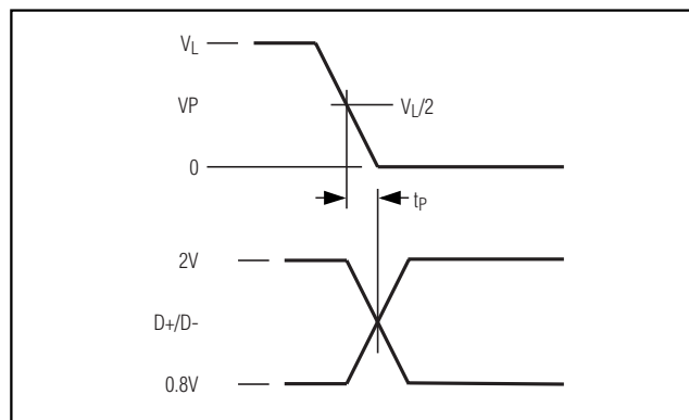
Figure 2. Mode 0 Timing
