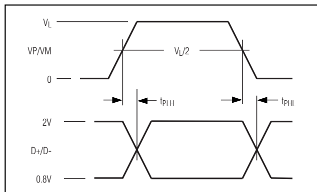
Figure 3. Mode 1 Timing
