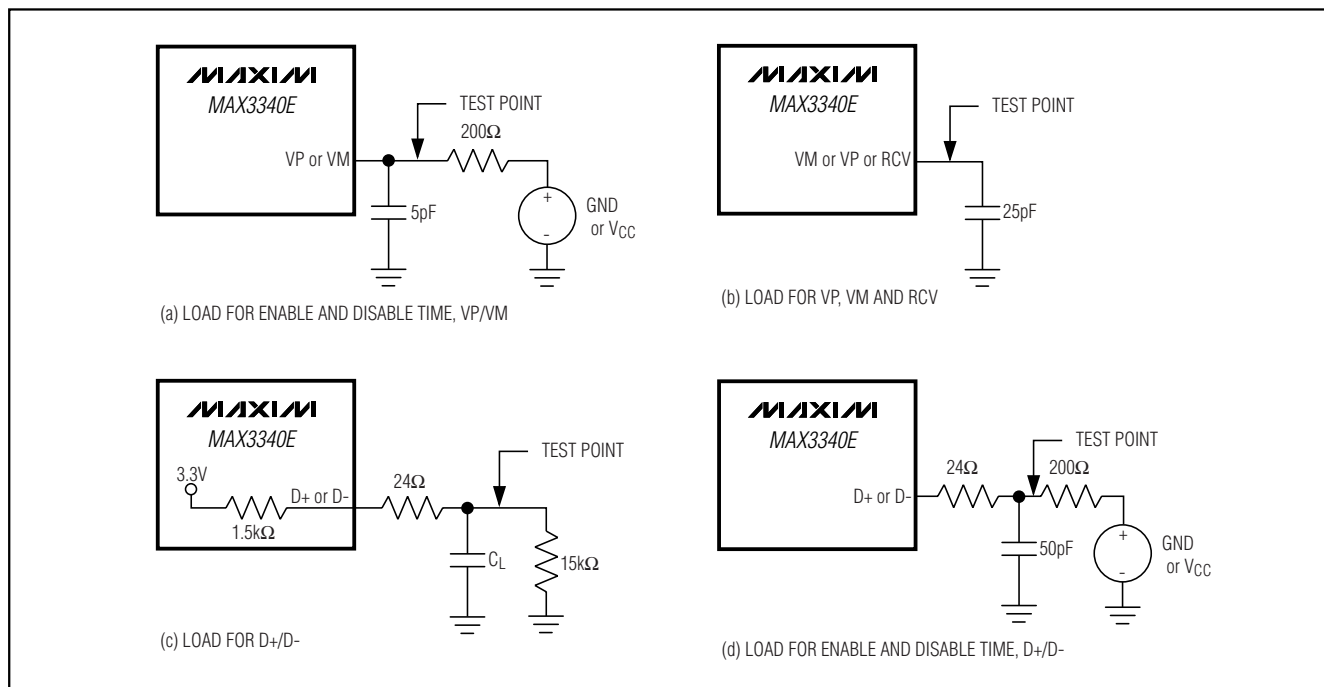
Figure 4. Test Circuits
