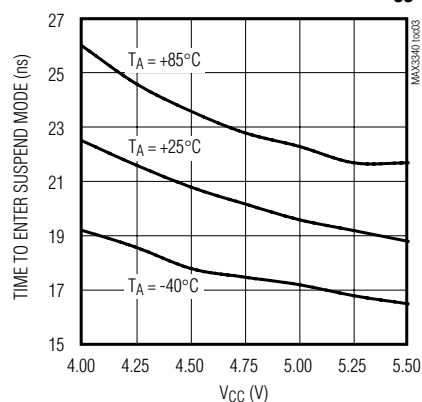
TIME TO ENTER SUSPEND MODE vs. V_{CC}
