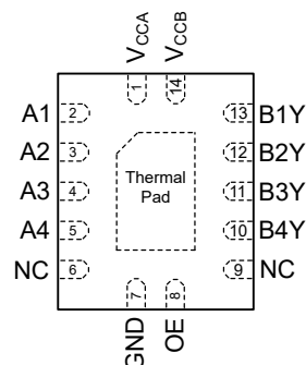
Figure 6-2. BQA Package 14-Pin VQFN Transparent Top View
