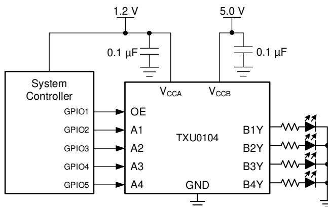
Figure 10-1. TXU0104 LED Driver Application
