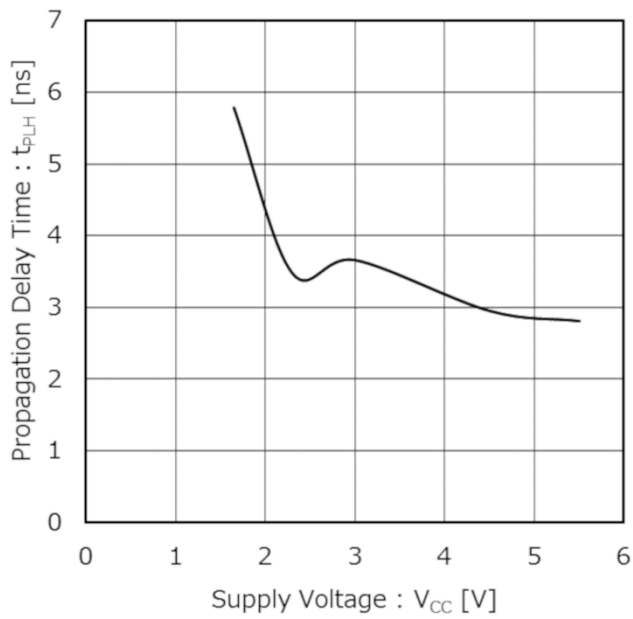
Figure 1. Propagation Delay Time: t_{PLH} vs Supply Voltage: V_{CC} ( T_a = 25^\circ\text{C} )
