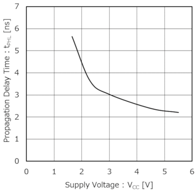
Figure 3. Propagation Delay Time: t_{PHL} vs Supply Voltage: V_{CC} ( T_a = 25^\circ\text{C} )
