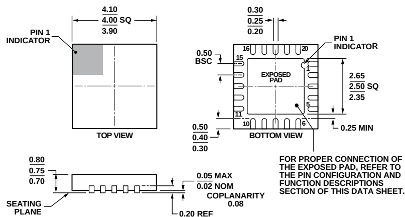
Figure 38. 20-Lead Lead Frame Chip Scale Package [LFCSP] 4 mm × 4 mm Body and 0.75 mm Package Height (CP-20-10) Dimensions shown in millimeters
