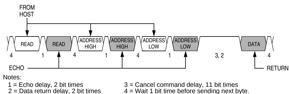
Figure 13-10. Read Transaction
