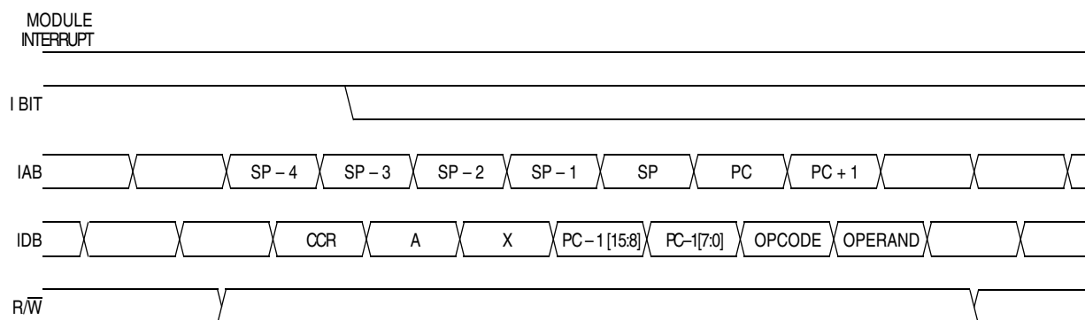
Figure 10-9. Interrupt Recovery
