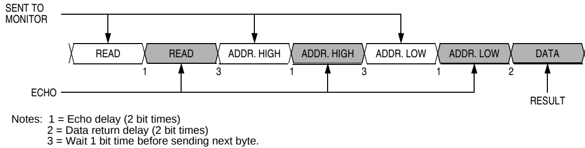
Figure 13-8. Read Transaction
