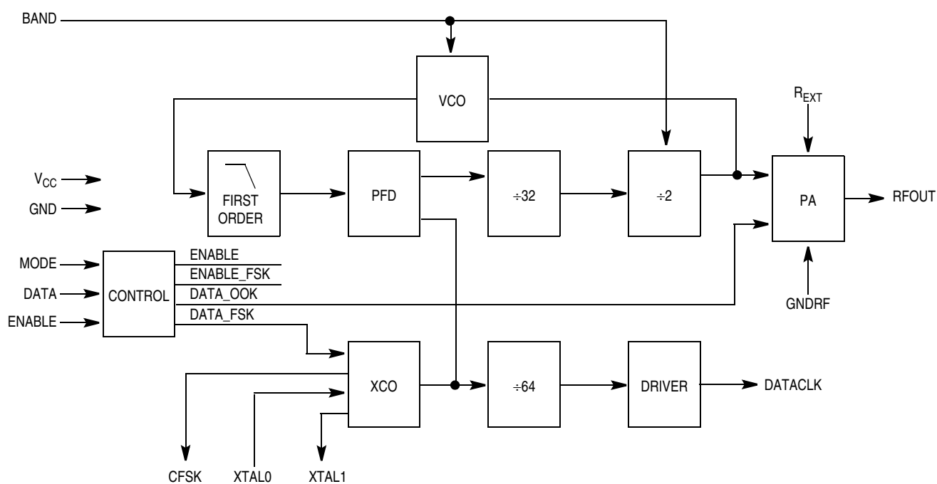
Figure 12-1. Simplified Integrated RF Module Block Diagram
