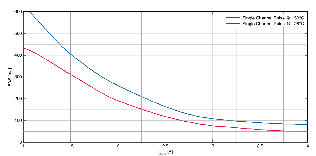
Figure 10 Maximum Energy Dissipation Single Pulse for a Single Channel, T_{j\_START} = 150^\circ\text{C} ; V_S = 28\text{ V}
