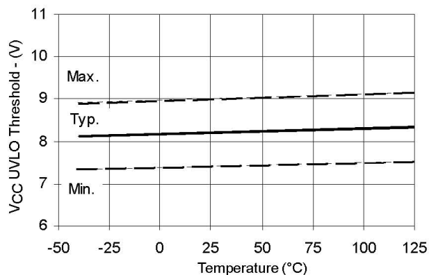
Figure 21B. V_{CC}|V_{BS} Undervoltage Threshold(-) vs. Temperature
