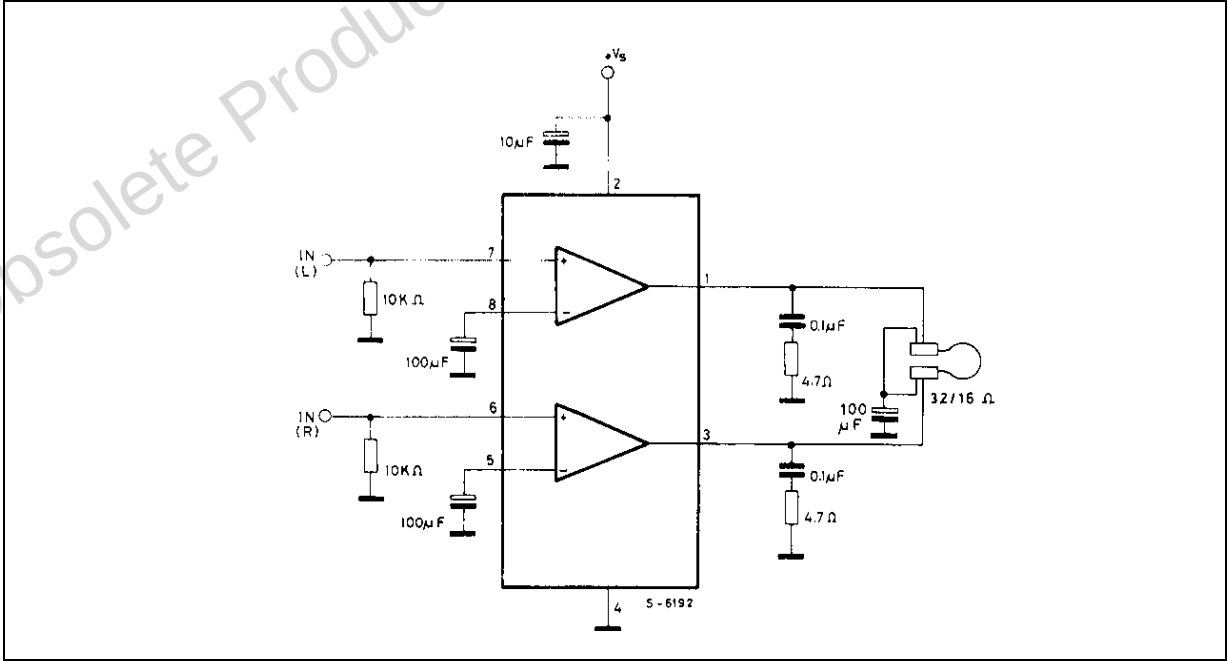
Figure 20 : Low Cost Application in Portable Players (using only one 100 \mu F output capacitor)
