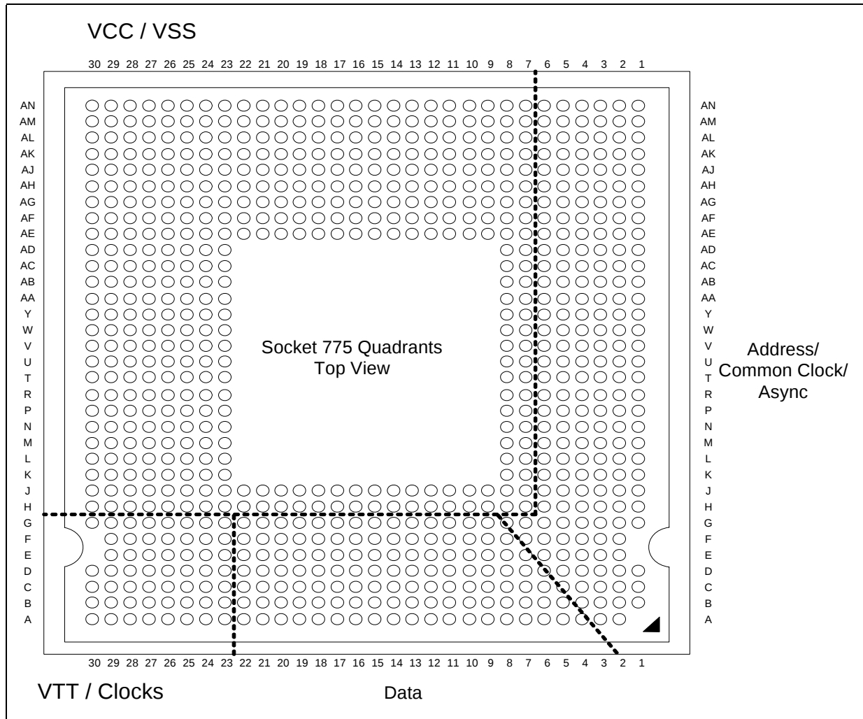
Figure 3-6. Processor Land Coordinates and Quadrants (Top View)
