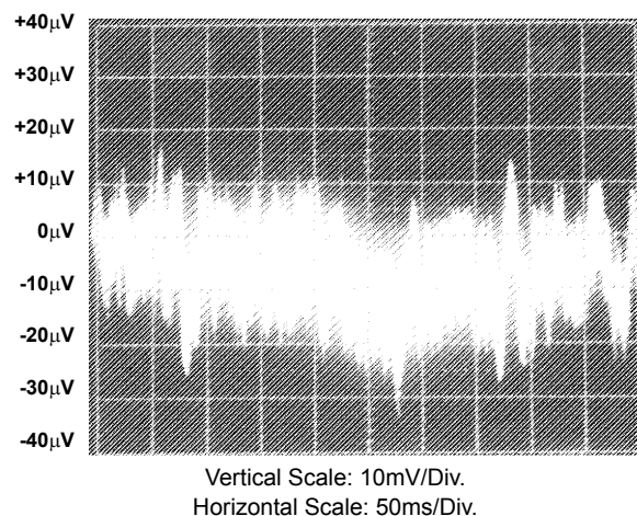
FIGURE 11. BROADBAND NOISE (0.1Hz TO 1MHz)
