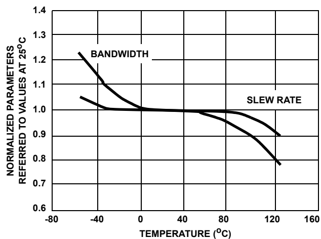
FIGURE 18. NORMALIZED AC PARAMETERS vs TEMPERATURE
