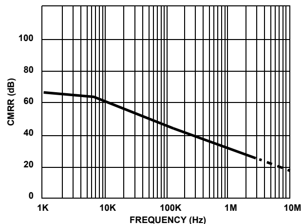
FIGURE 12. COMMON MODE REJECTION RATIO vs FREQUENCY
