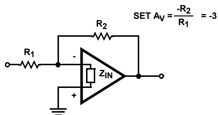
FIGURE 6. STABILIZATION USING Z_{IN}
