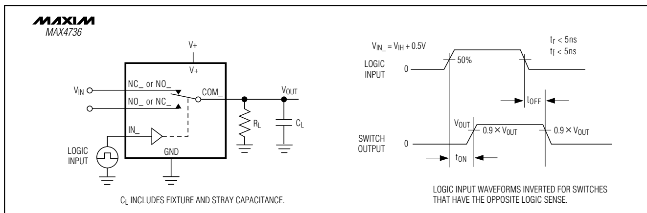
Figure 1. Switching Time
