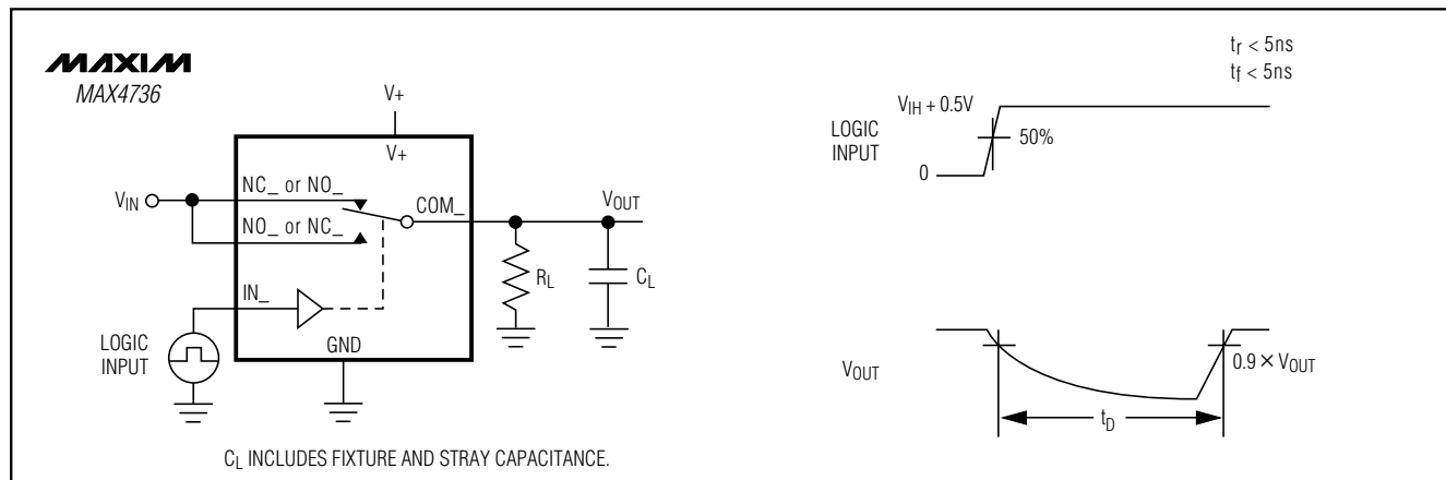
Figure 2. Break-Before-Make Interval
