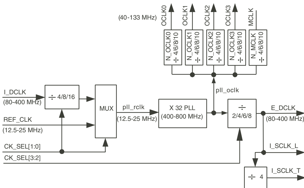
Figure 30. Clock generator
