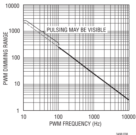
Figure 8. Dimming Ratio vs Frequency
