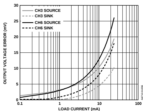
Figure 7. Output Voltage Error vs. Load Current
