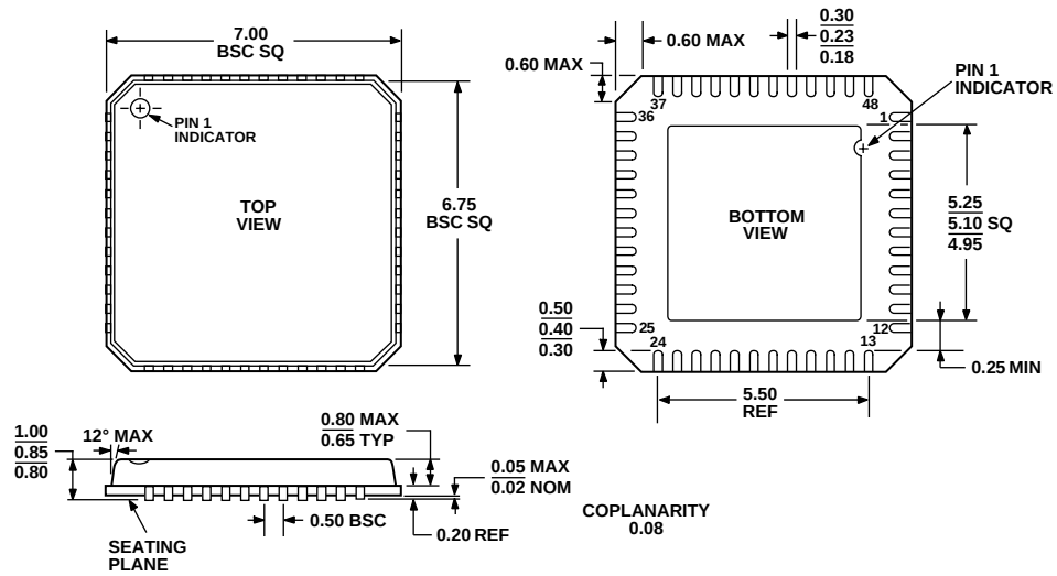
Figure 31. 48-Lead Frame Chip Scale Package [LFCSP] (CP-48)
