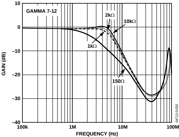
Figure 27. Frequency Response vs. Resistive Loading
