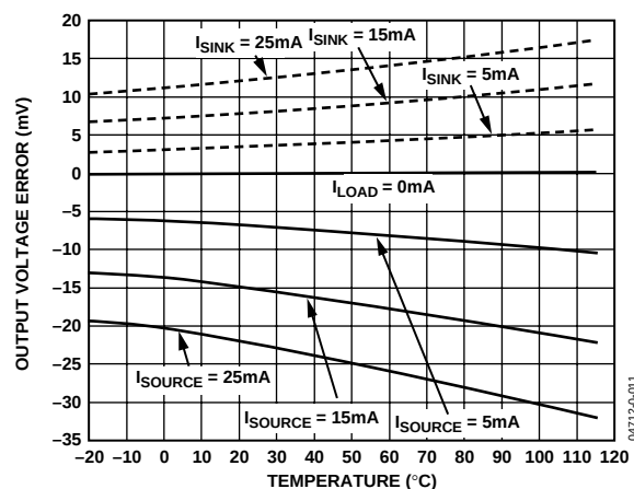
Figure 5. Output Voltage Error vs. Temperature
