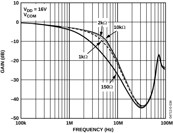
Figure 28. Frequency Response vs. Resistive Loading
