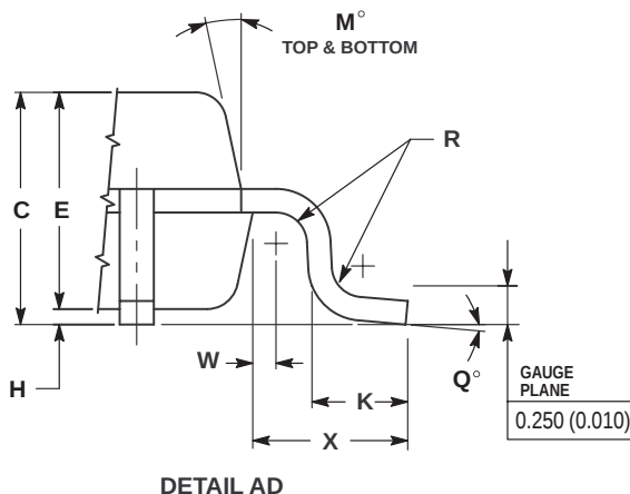
DETAIL AD
