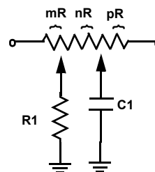
PROGRAMMABLE LADDER NETWORKS
