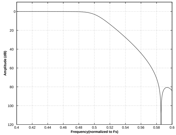
Figure 48. Double-Speed (fast) Transition Band
