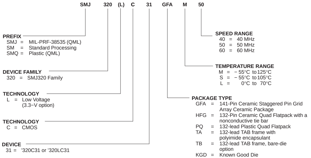
Figure 34. Device Nomenclature
