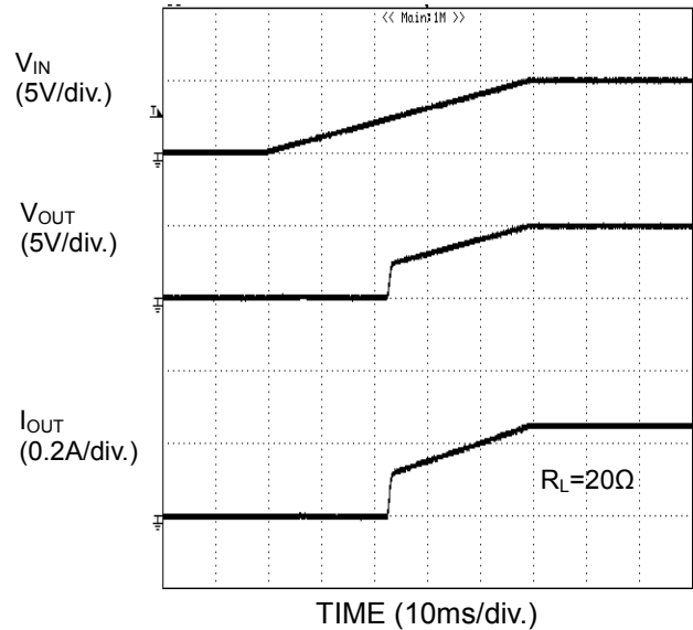
Figure 35. UVLO Response when Increasing V<sub>IN</sub>
