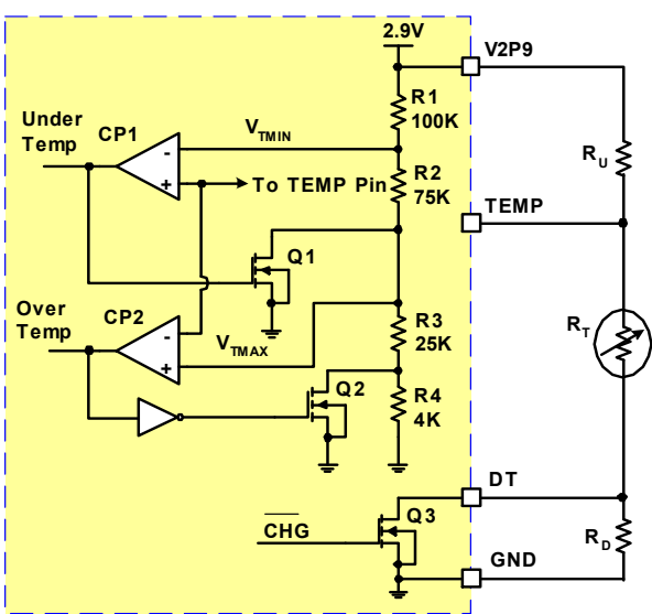
FIGURE 6. THE INTERNAL AND EXTERNAL CIRCUIT FOR THE NTC INTERFACE
