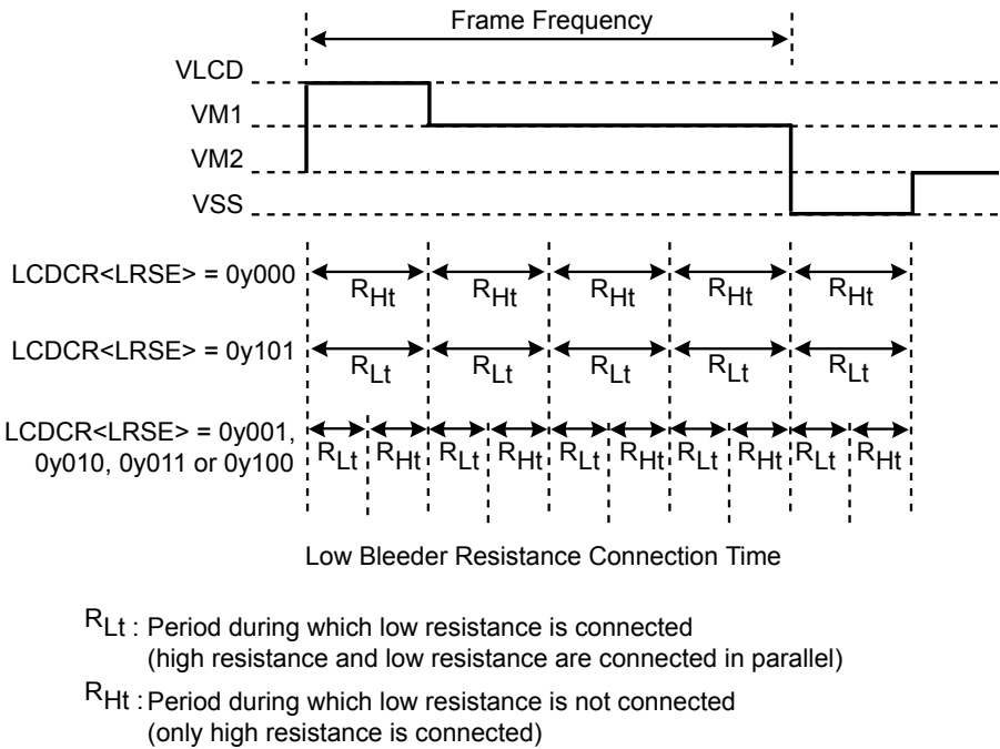
Figure 17-3 Bleeder Resistance Selection by LCDCR2<LRSE> (1/4 Duty, 1/3 Bias)
