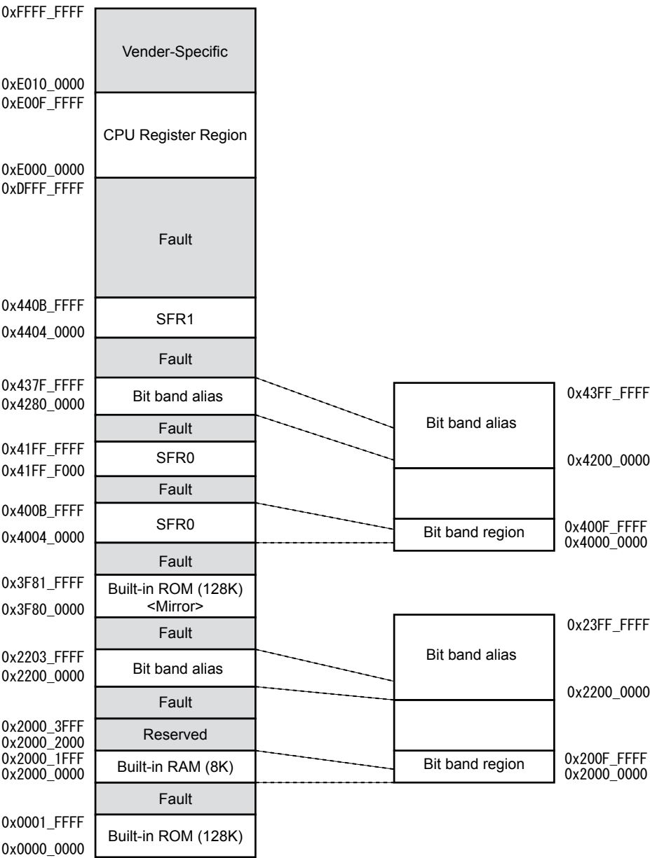
Figure 4-1 Memory Map
