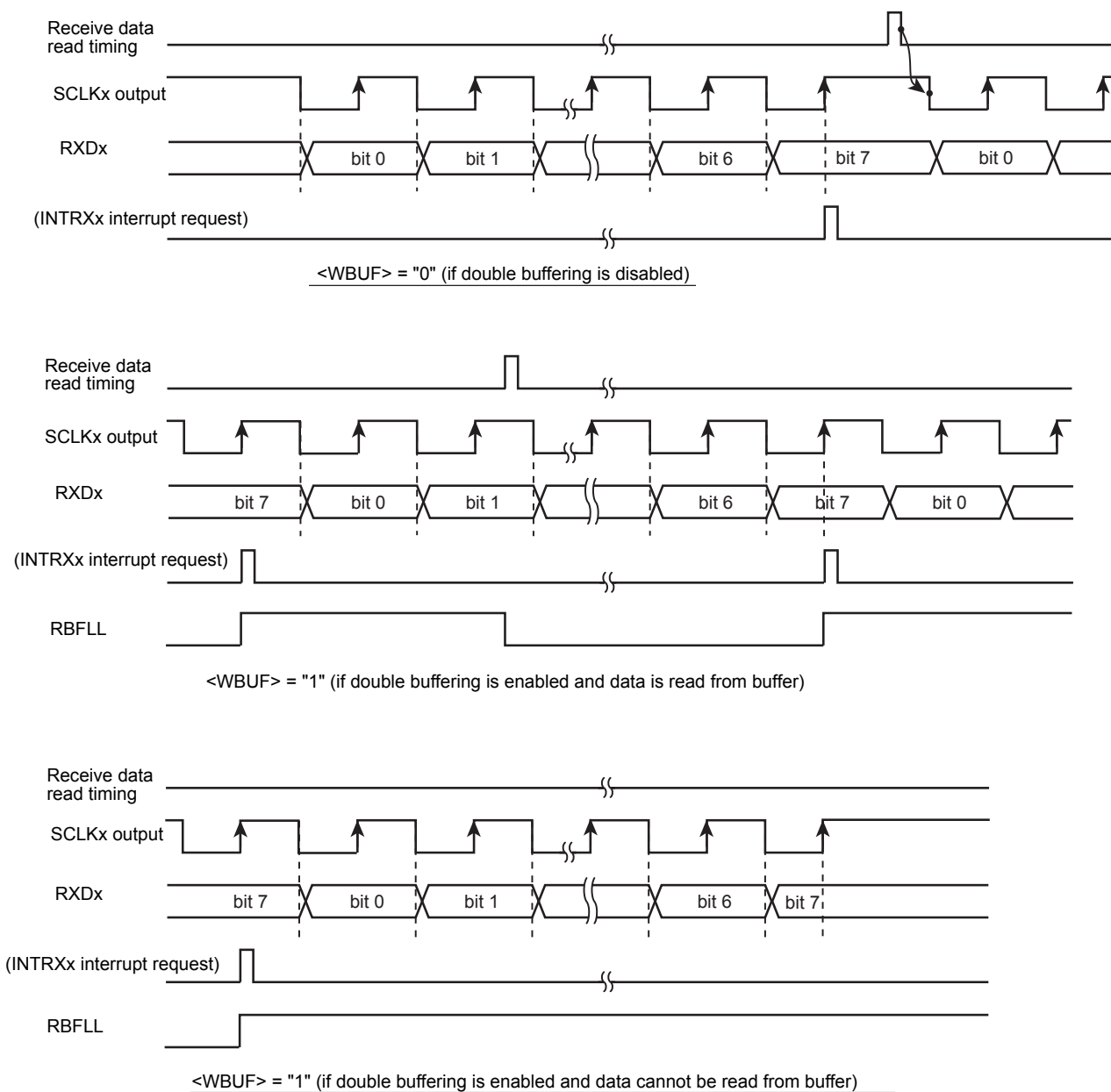
Figure 11-15 Receive Operation in the I/O Interface Mode (SCLK Output Mode)
