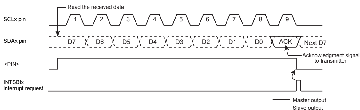
Figure 12-9 \langle BC[2:0] \rangle = "000" , \langle ACK \rangle = "1" (Receiver Mode)
