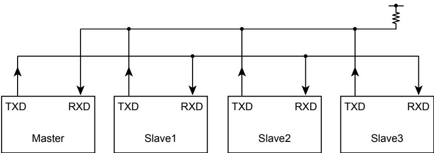
Figure 11-19 Serial Links to Use Wake-up Function
