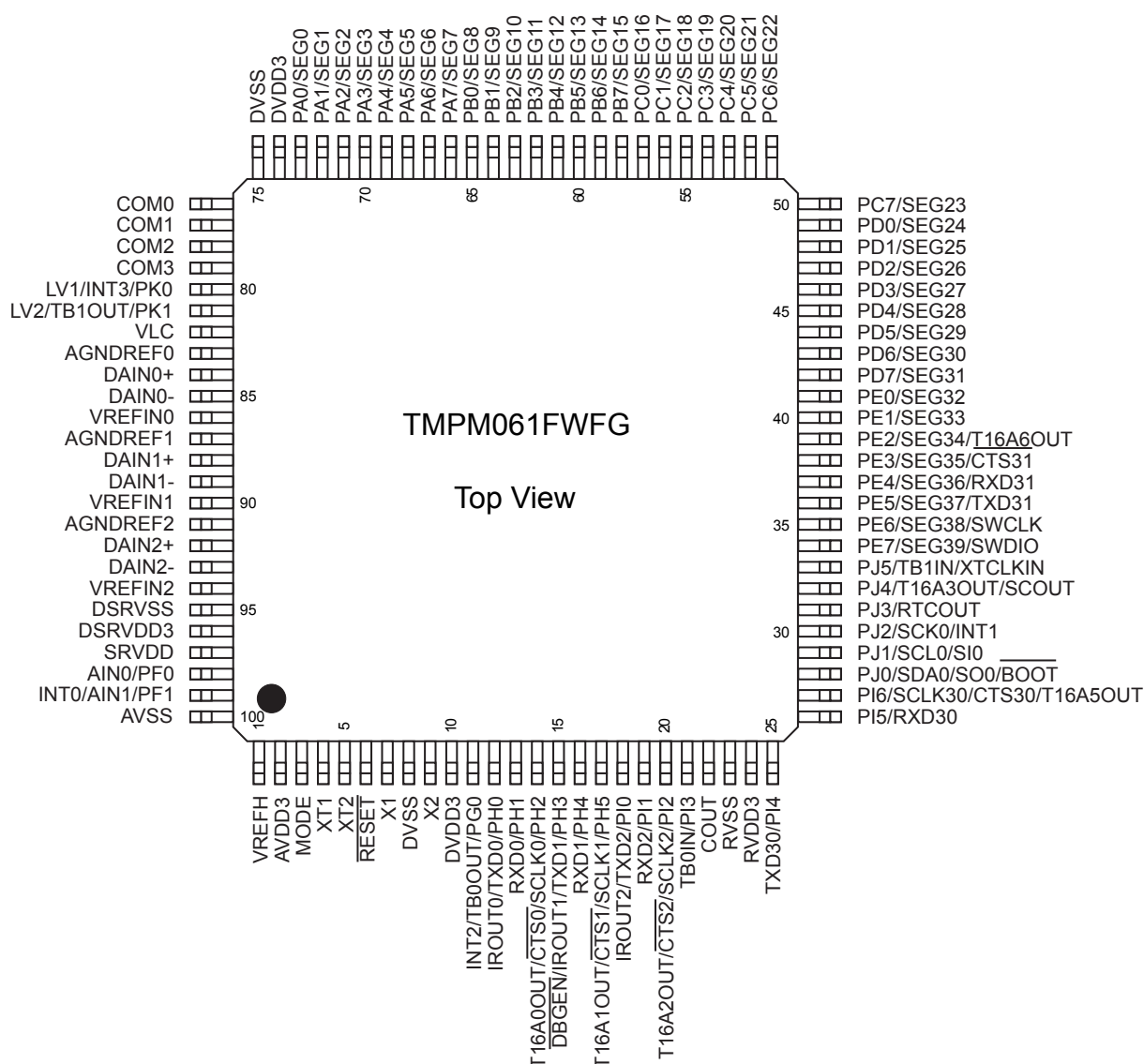
Figure 1-2 Pin Layout
