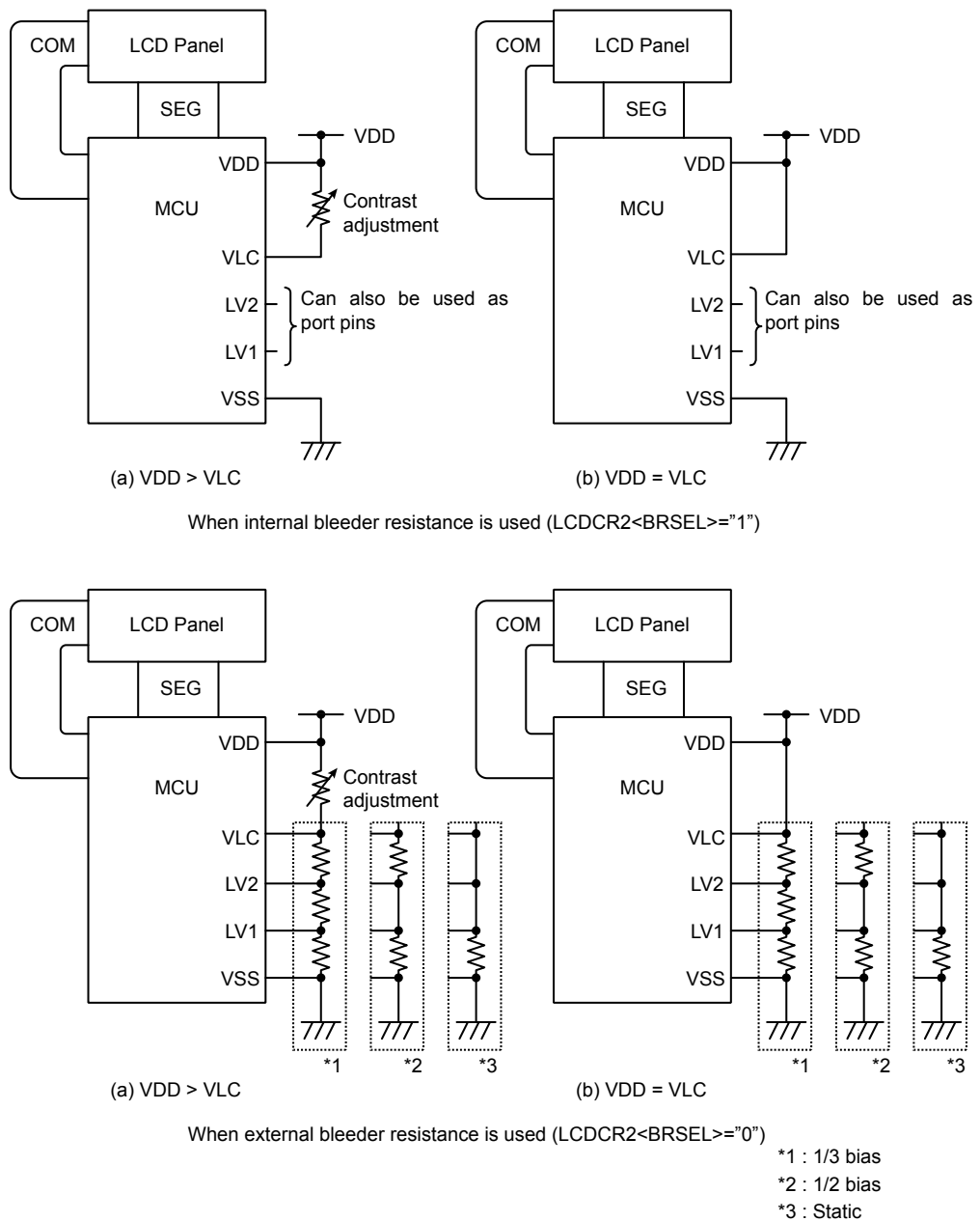
Figure 17-4 Connection Examples
