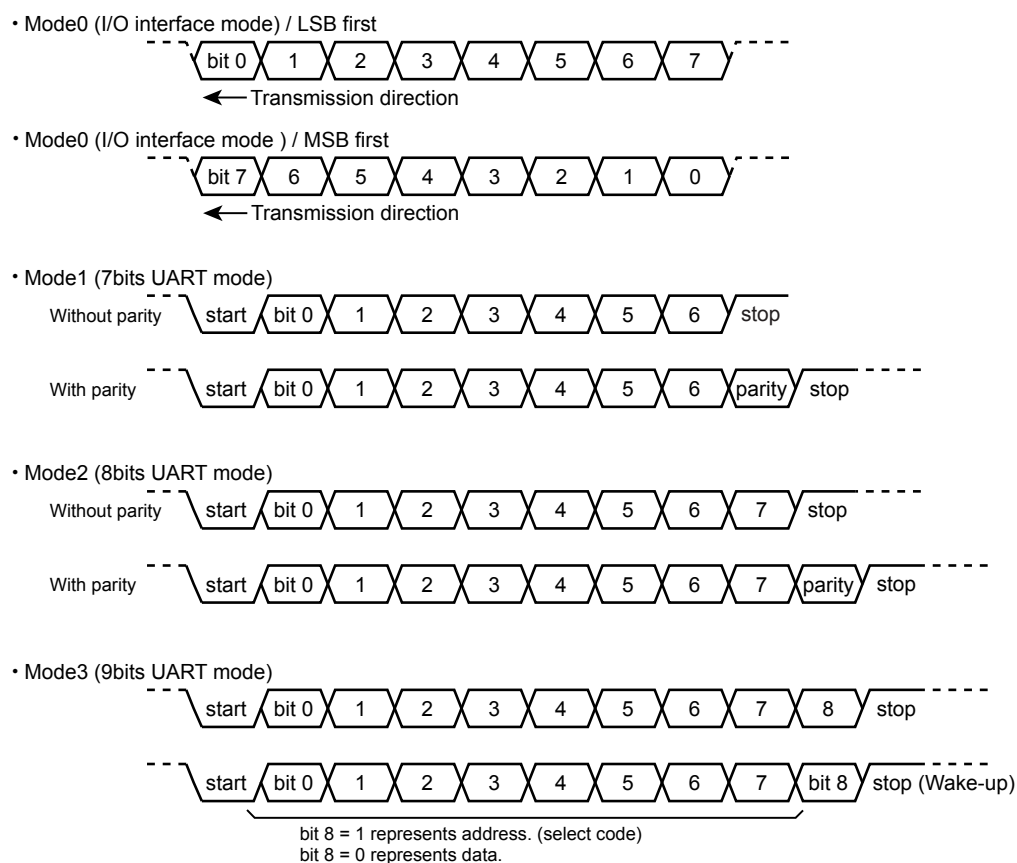
Figure 11-2 Data Format
