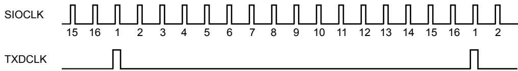
Figure 11-6 Generation of Transmission Clock
