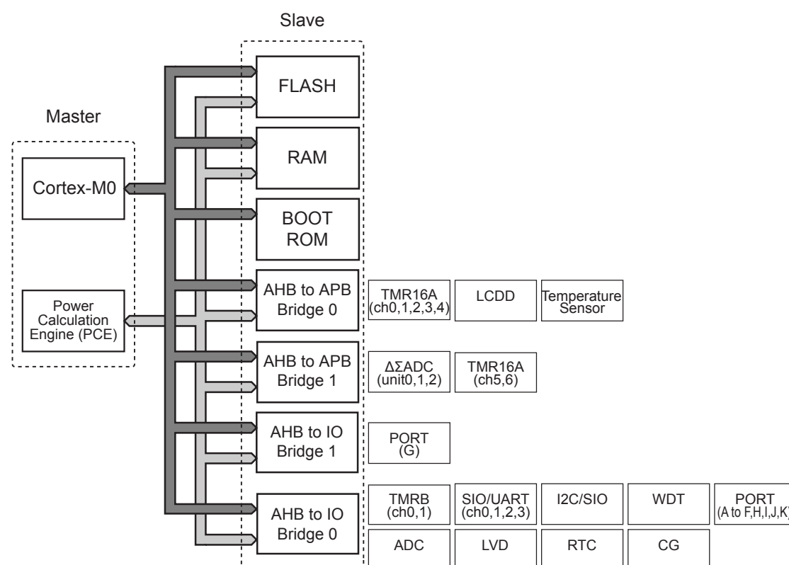
Figure 4-2 Bus structure
