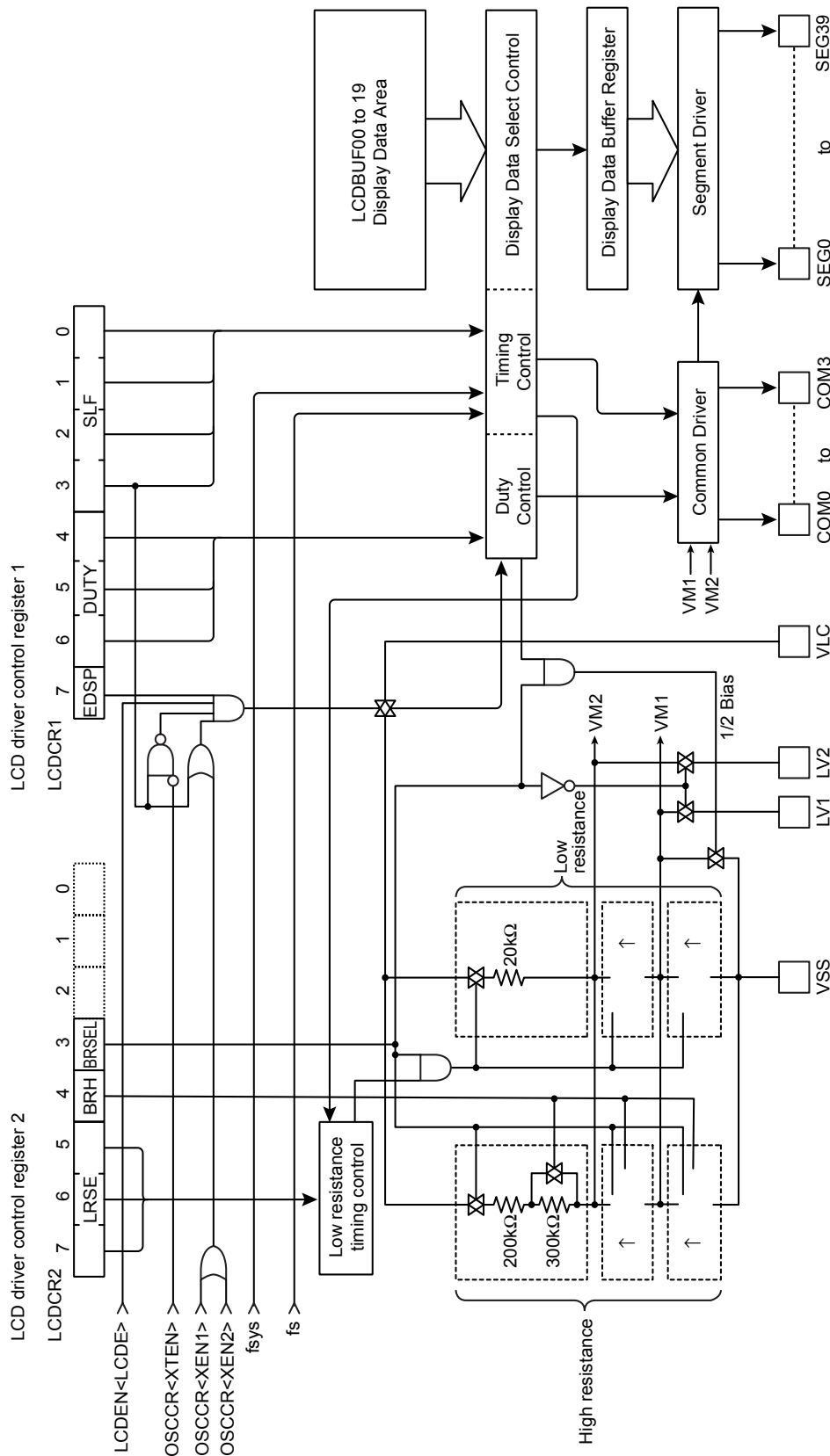
Figure 17-1 LCD Driver
