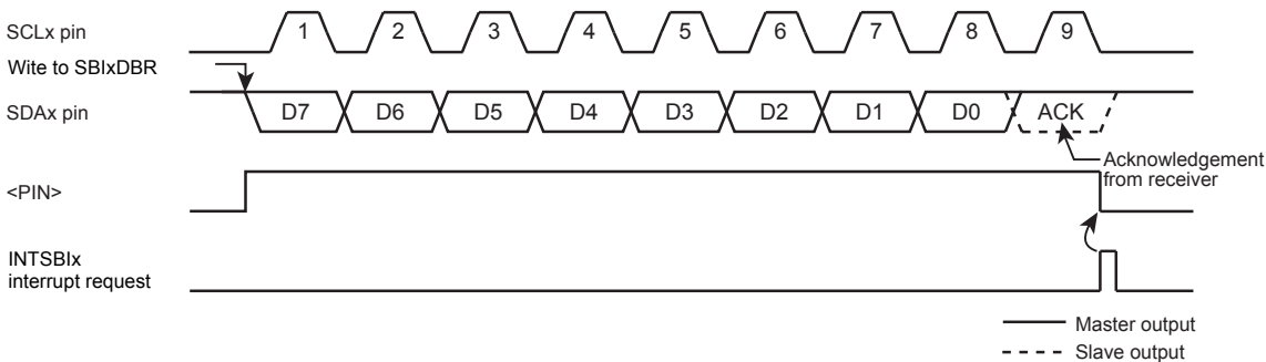
Figure 12-8 <BC[2:0]>= "000", <ACK>= "1" (Transmitter Mode)
