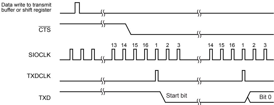
Figure 11-9 \overline{\text{CTS}} Signal timing
