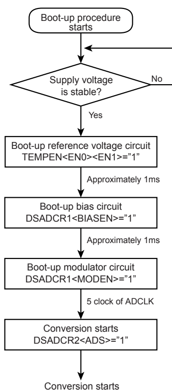
Figure 14-2 Boot-up procedure
