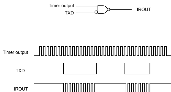
Figure 11-10 Output signal using IR carrier pulse
