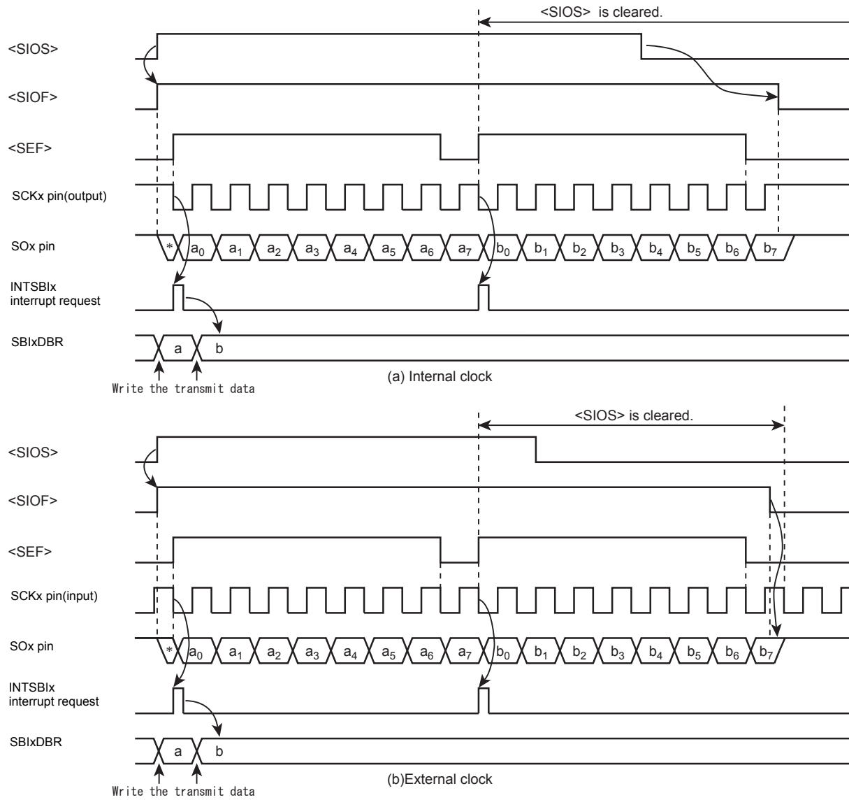
Figure 12-16 Transmit Mode
