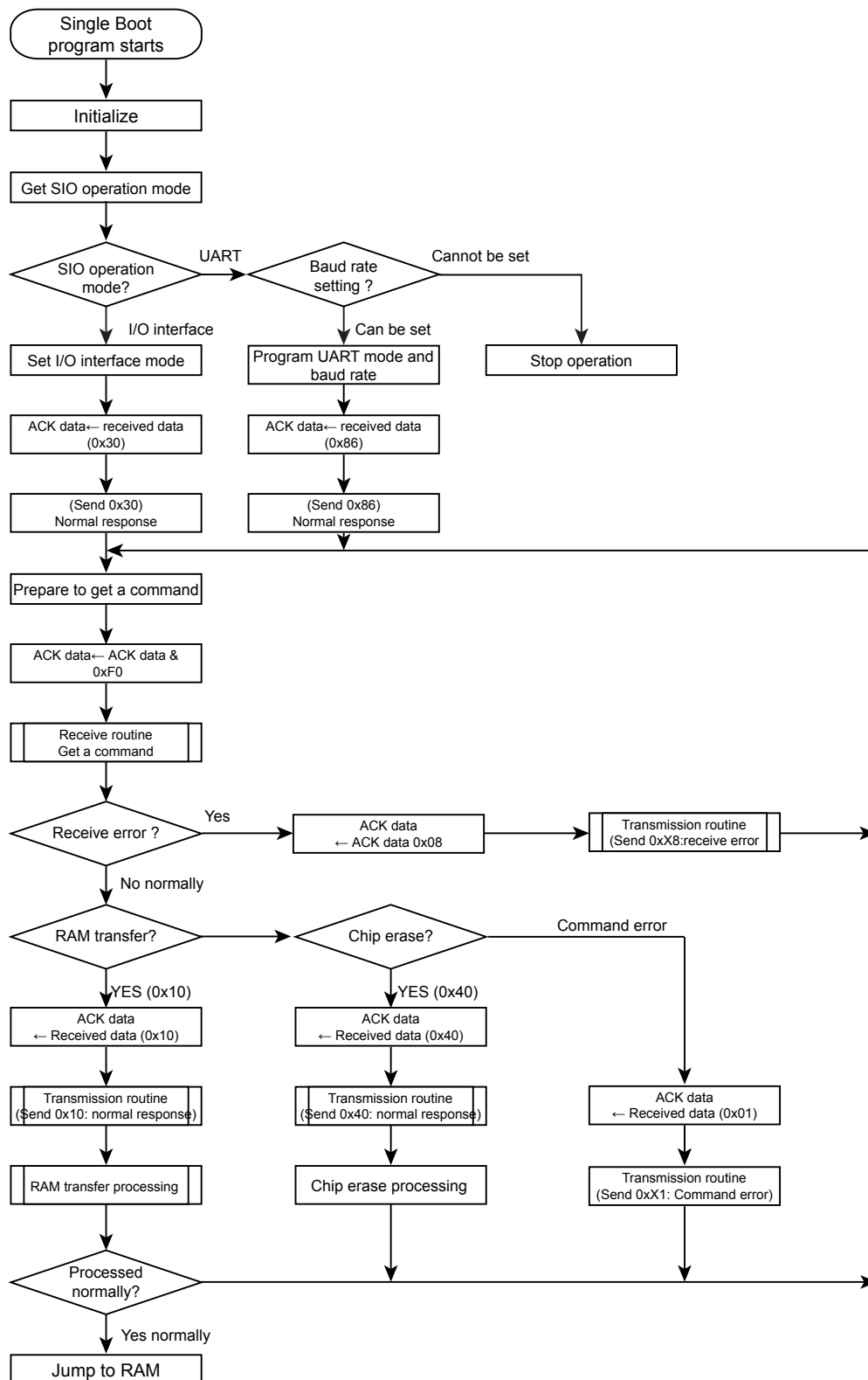
Figure 20-11 Boot program whole flowchart
