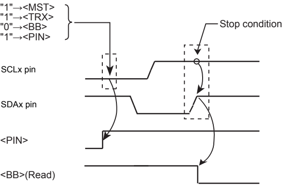
Figure 12-11 Generating the Stop Condition
