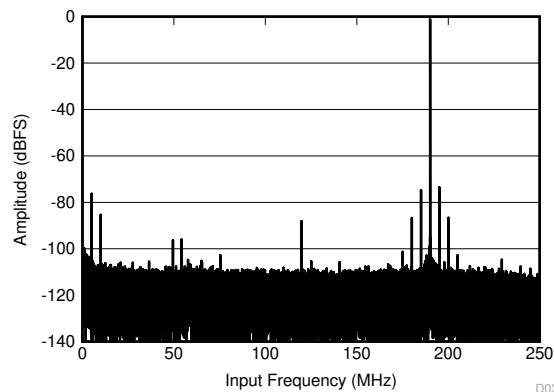
Figure 6-31. Power-Supply Rejection Ratio FFT for 50-mV Noise on AVDD Supply
