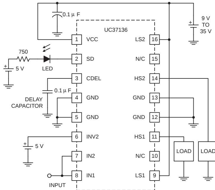
Figure 1. Both Switches Configured as High Side, Switch 2 Inverted with Respect to Switch 1
