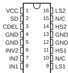
DP, M, OR NP PACKAGES (TOP VIEW)
