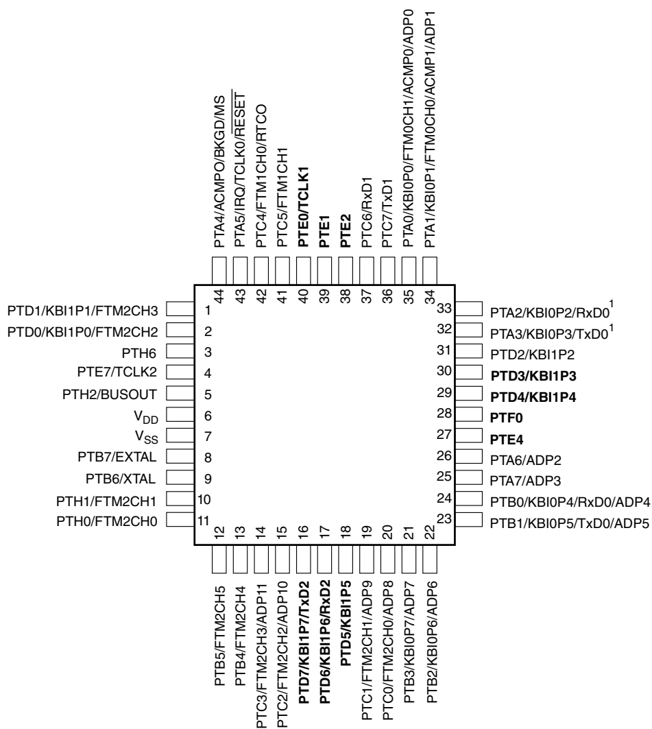
Figure 14. MC9S08PL60 44-pin LQFP package
