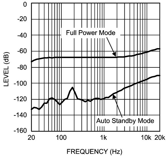
PSRR vs Frequency V_{DD} = 1.6V , R_L = 16\Omega
