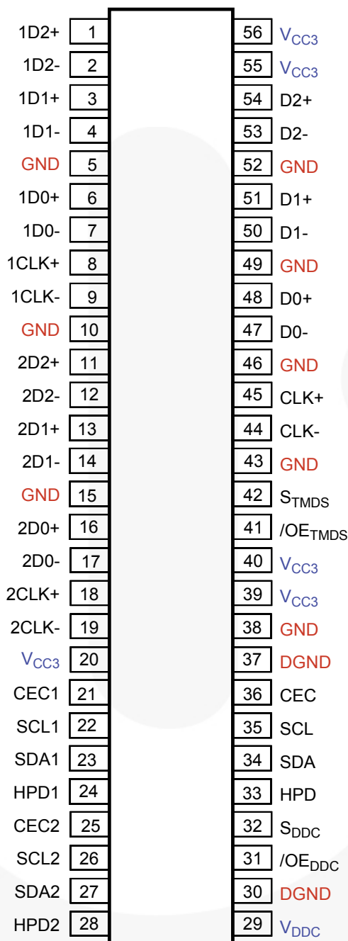
Figure 3. Pin Assignments
