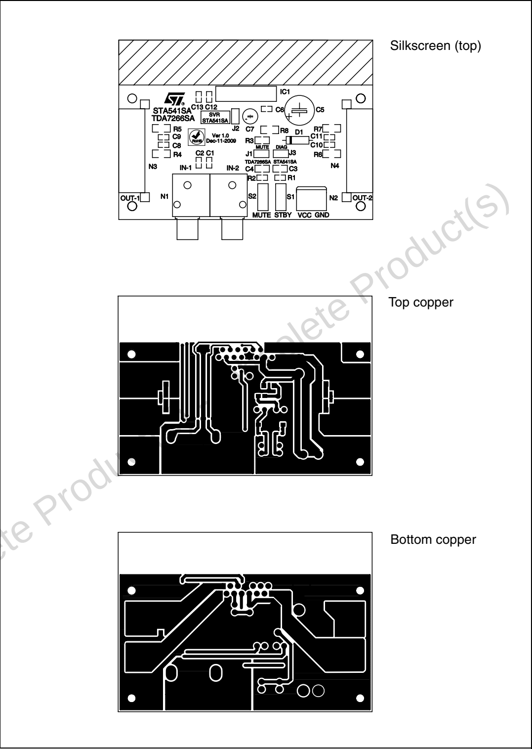
Figure 16. PCB layout
