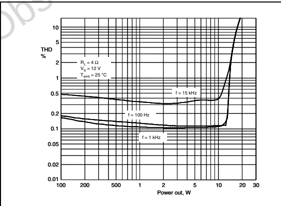
Figure 6. Total harmonic distortion vs output power
