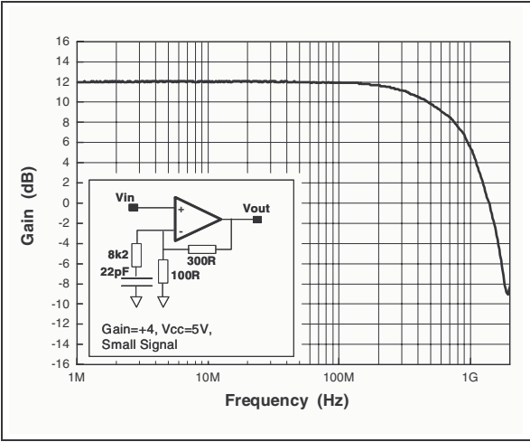
Figure 6. Compensation, gain=+4
