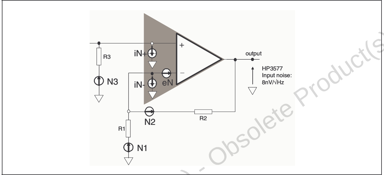
Figure 33. Noise model
