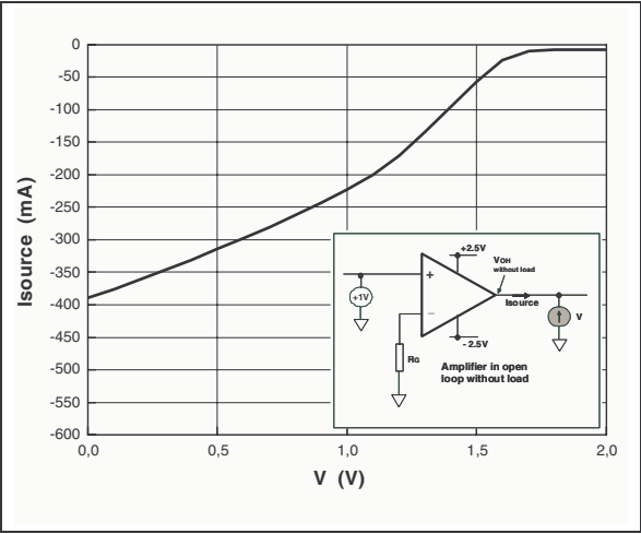
Figure 18. Isource
