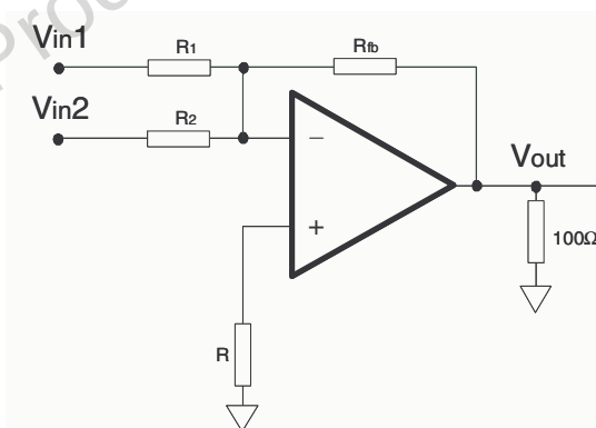
Figure 34. Inverting summing amplifier (using evaluation board SO8_S_MULTI)
