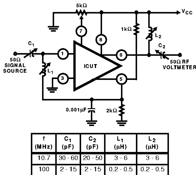
FIGURE 9. AGC RANGE TEST CIRCUIT (DIFFERENTIAL AMPLIFIER) FOR CA3028A AND CA3028B
