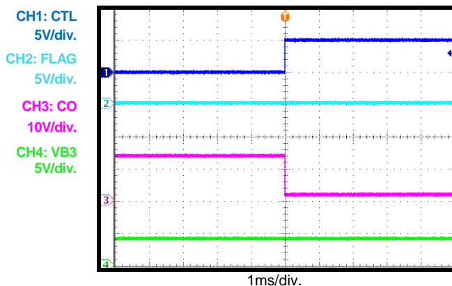
CTL Response
