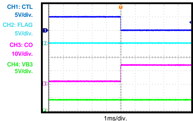
CTL Response
