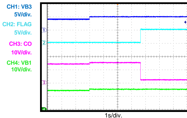
OVP Response
