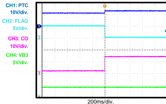
CTL Response
