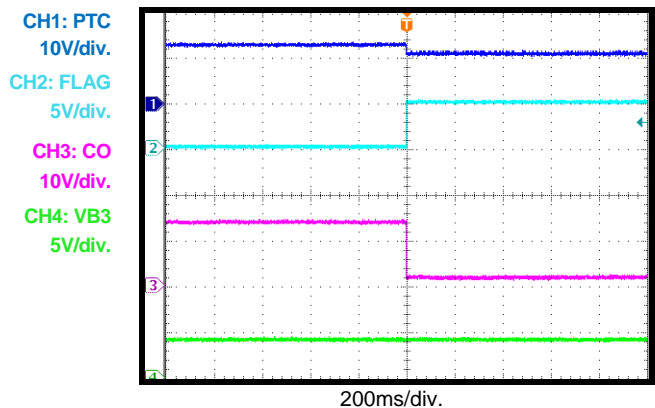
PTC Delay
