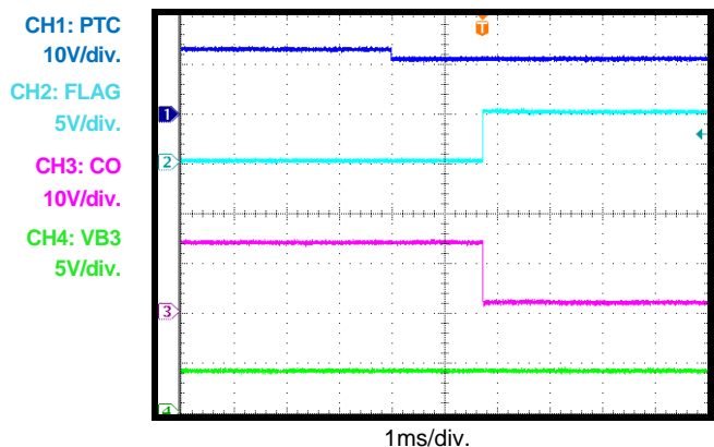
PTC Delay
