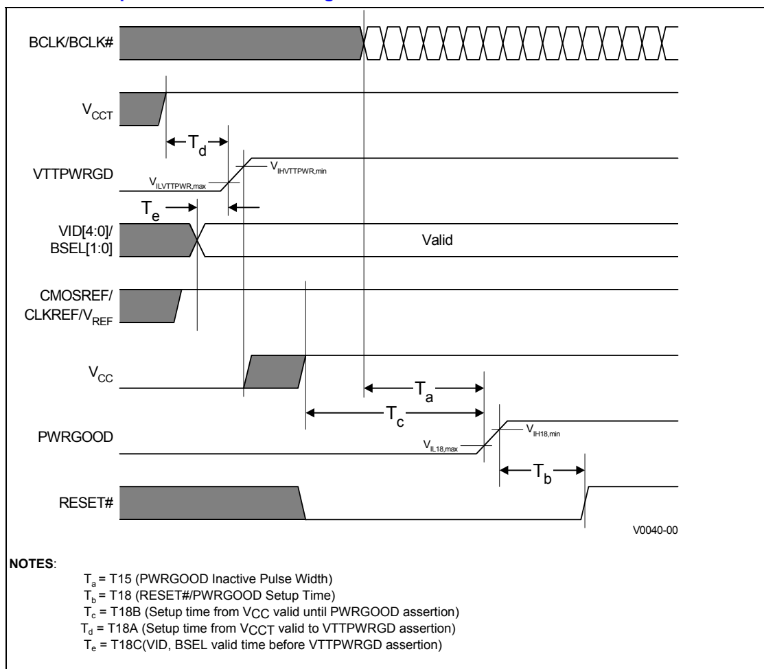
Figure 15. Power-on Sequence and Reset Timings
