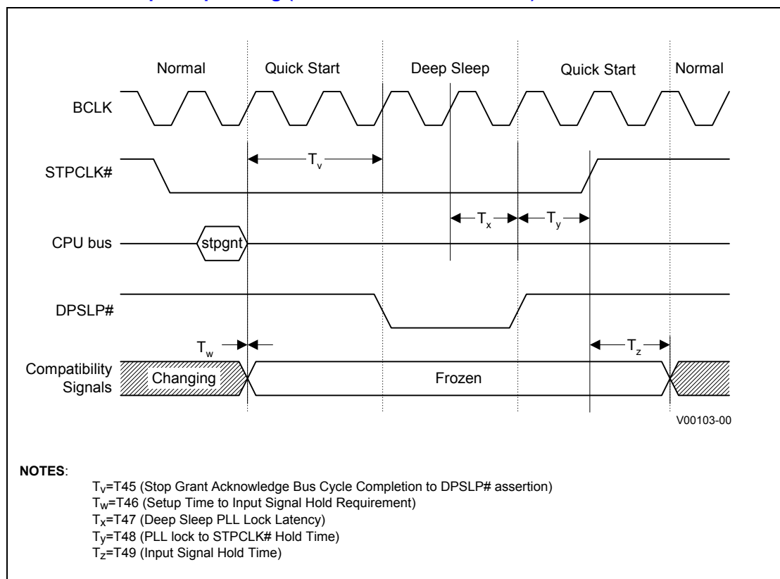
Figure 21. Quick Start/Deep Sleep Timing (DPSP# Assertion Method)
