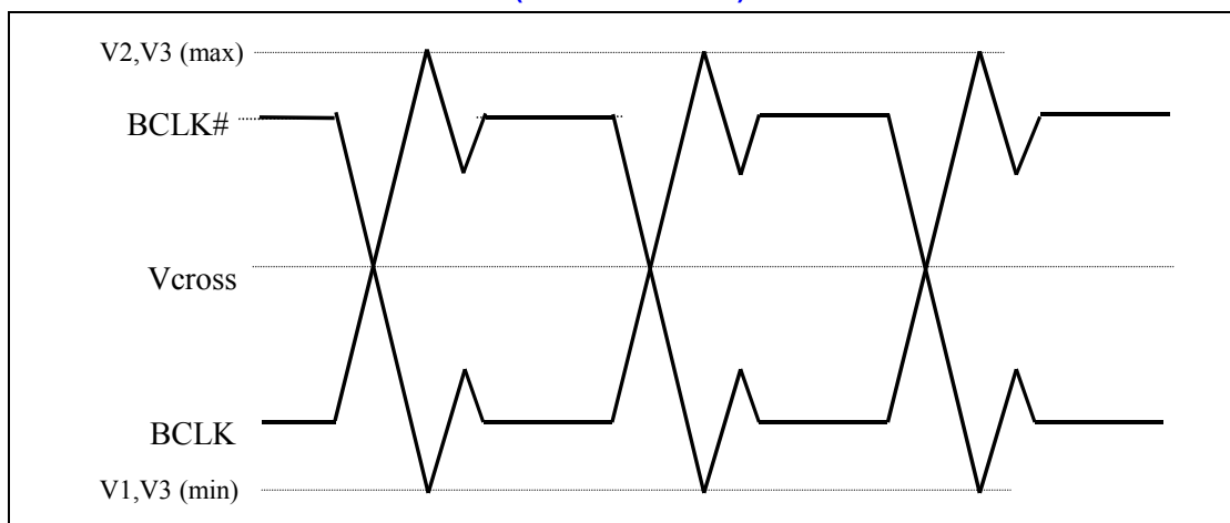
Figure 10. Differential BCLK/BCLK# Waveform (Common Mode)
