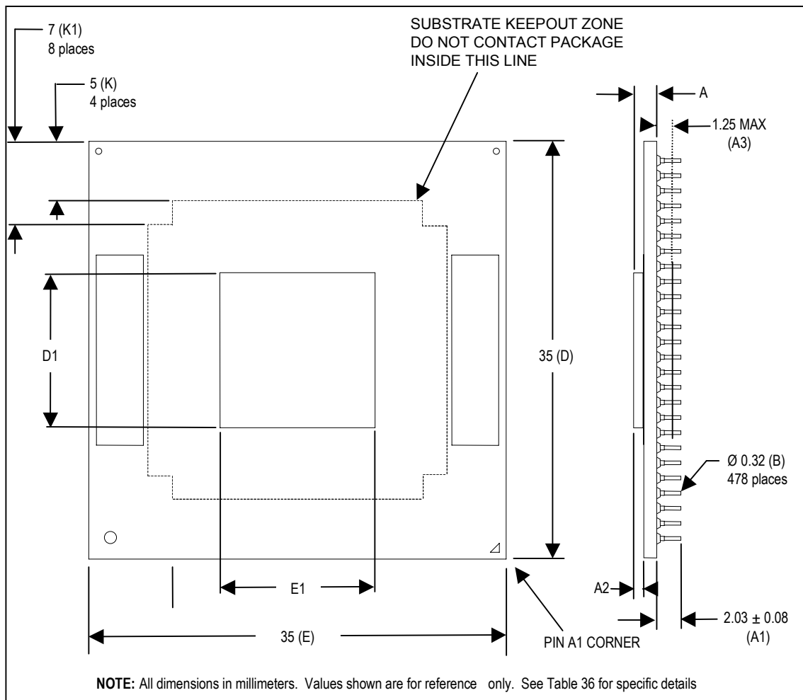
Figure 26. Socketable Micro-FCPGA Package - Top and Side View
