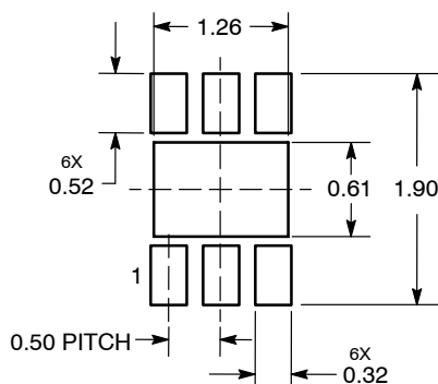
BOTTOM VIEW + 0.05 C NOTE 3 SOLDERMASK DEFINED MOUNTING FOOTPRINT*
