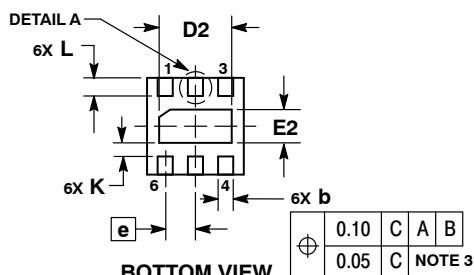
BOTTOM VIEW + 0.05 C NOTE 3 SOLDERMASK DEFINED MOUNTING FOOTPRINT*
