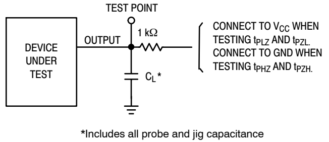
Figure 7. Test Circuit
