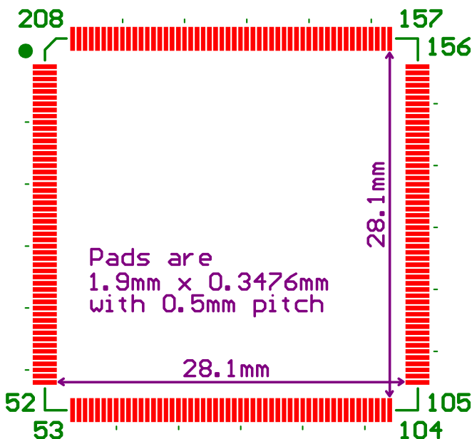
Figure 24. QFP-132 Typical PCB Foil Pattern (0.006" gap between pads)
