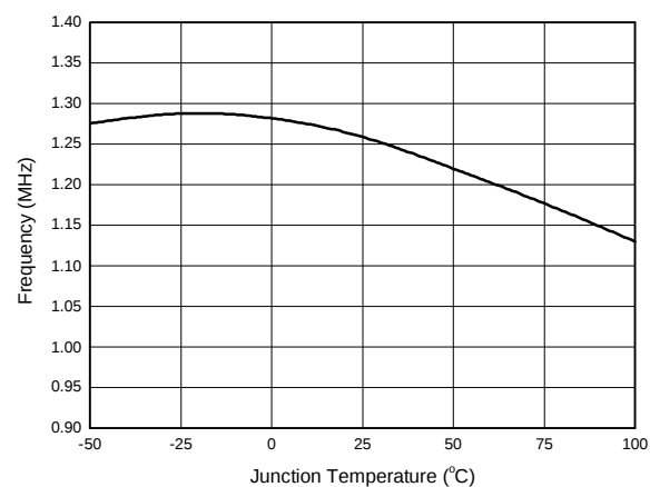
Figure 11. Switch Frequency vs. Junction Temperature
