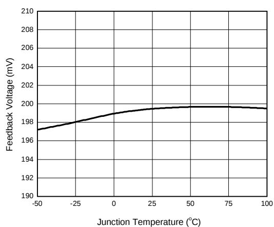
Figure 12. Feedback Voltage vs. Junction Temperature
