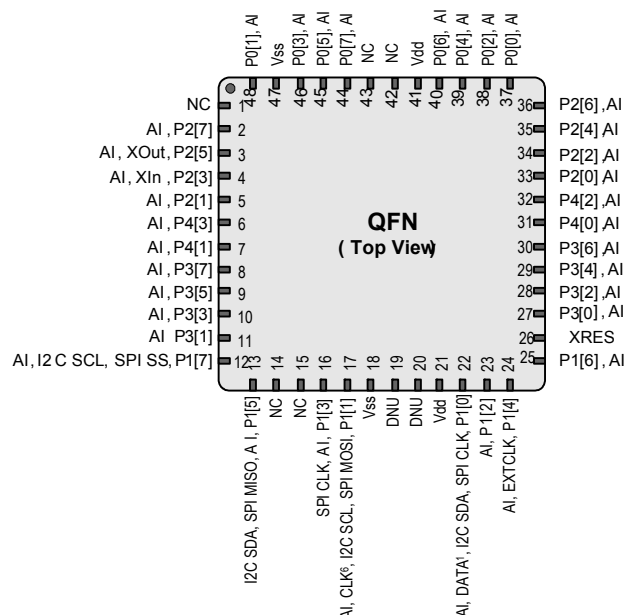
Figure 7. CY8C20636 PSoC Device
