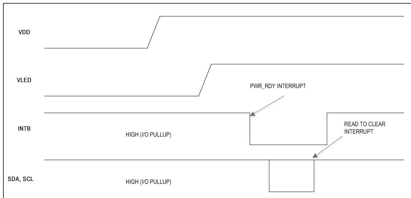
Figure 2: Power-Up Sequence of the Power Supply Rails
