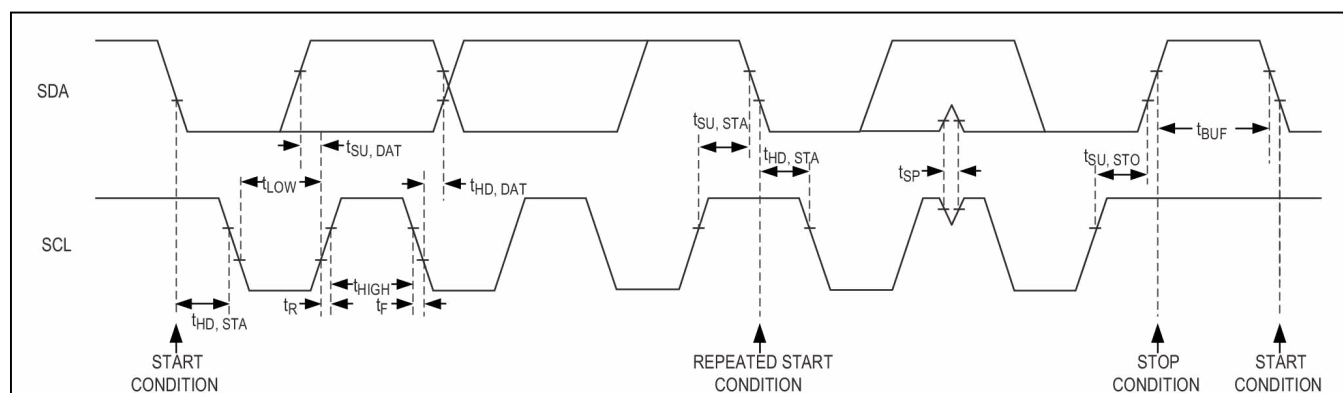
Figure 1. I²C-Compatible Interface Timing Diagram
