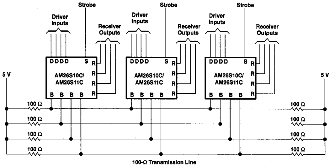
Figure 2. Party-Line System
