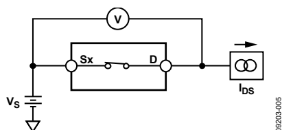
Figure 23. On Resistance
