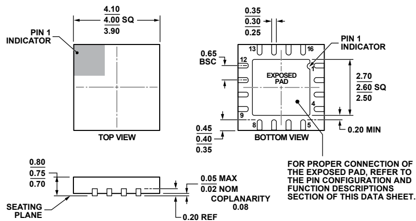
COMPLIANT TO JEDEC STANDARDS MO-220-WGGC. Figure 36. 16-Lead Lead Frame Chip Scale Package [LFCSP] 4 mm × 4 mm Body and 0.75 mm Package Height (CP-16-17) Dimensions shown in millimeters
